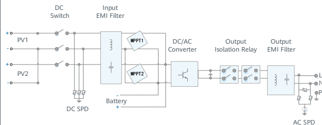
Circuit Diagram
